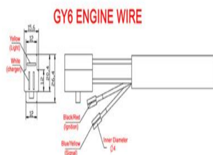
4-STROKE GY6 WIRE DIAGRAM
