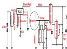
4-STROKE GY6 WIRE DIAGRAM
