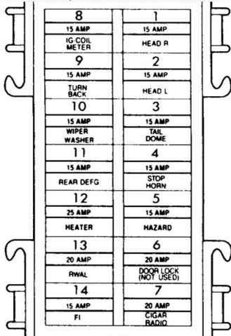
1992 Geo Tracker Fig. 1: Fuse Panel Identification Courtesy of GENERAL MOTORS CORP.
